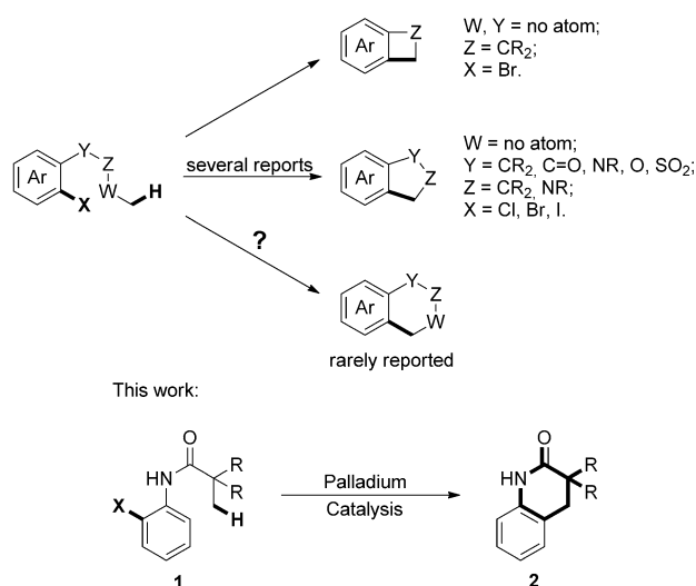
Figure 1. C(sp 3 )-H activation reactions that are initiated by oxidative addition.
